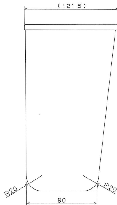
C部詳細 (S=2/1)
